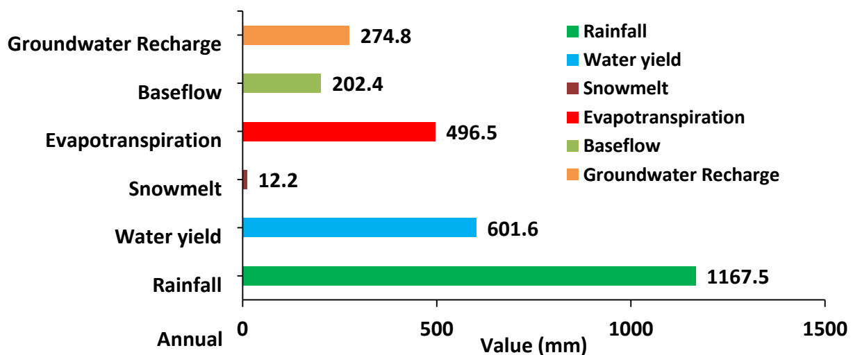
Figure 4.3: Average (1969-2006) Annual Water Balance of the Modeled Ganga Basin
