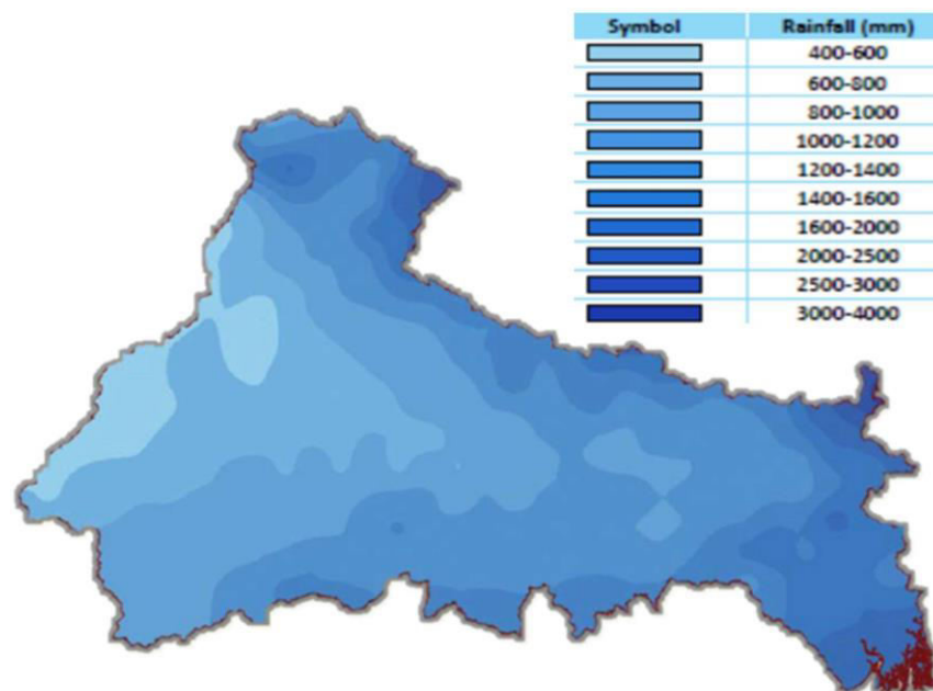
Figure 2.2a: Average Annual Rainfall in NRGB [from India-WRIS, 2012]
