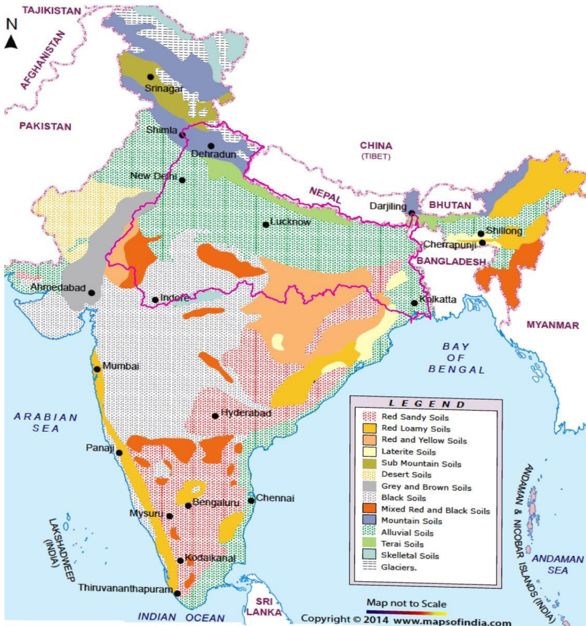
Figure 2.3c: Soil Map of NRGB [Adapted from: MapsofIndia.com, 2014b]
