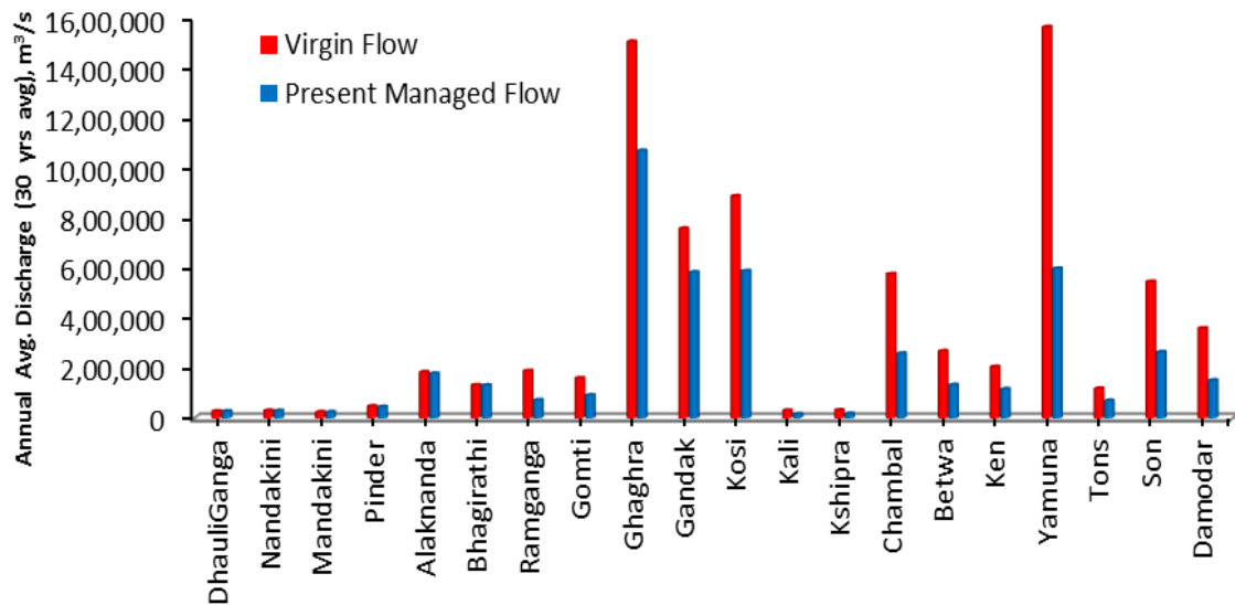
Figure 4.4: Annual Flow Contributions of Different Tributaries (sub-basins) to National River Ganga under Present Flow Conditions and under Virgin Flow Conditions
